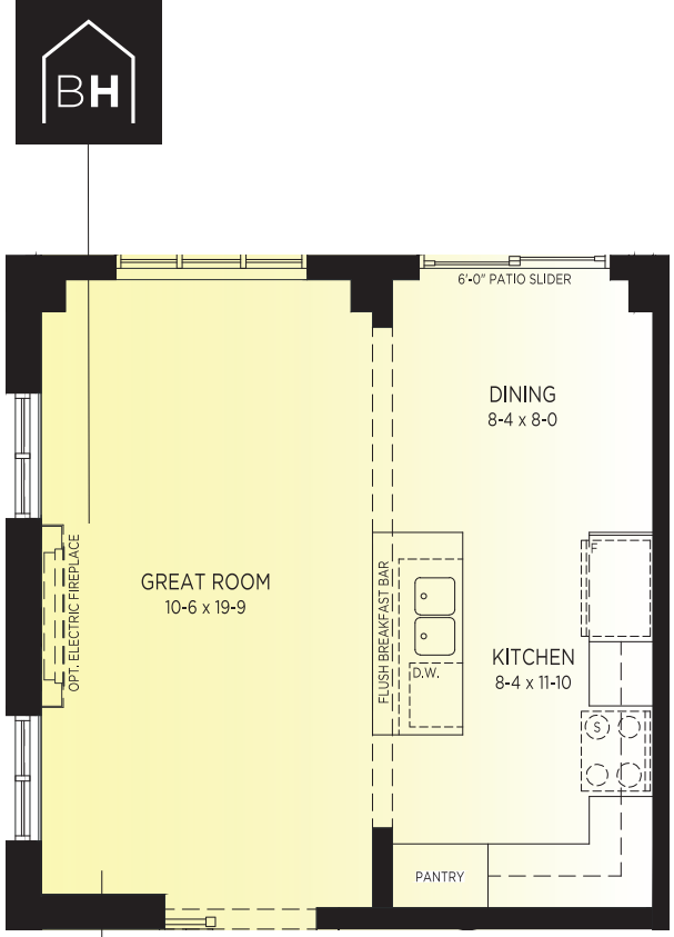
FLEXFIT GROUND FLOOR ALTERNATE KITCHEN LAYOUT
