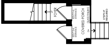
ELEV. A FIRST LEVEL FRONT
