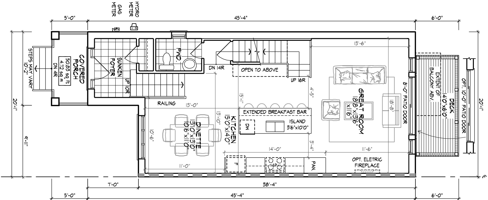
MAIN FLOOR PLAN ELEV. 'A'
