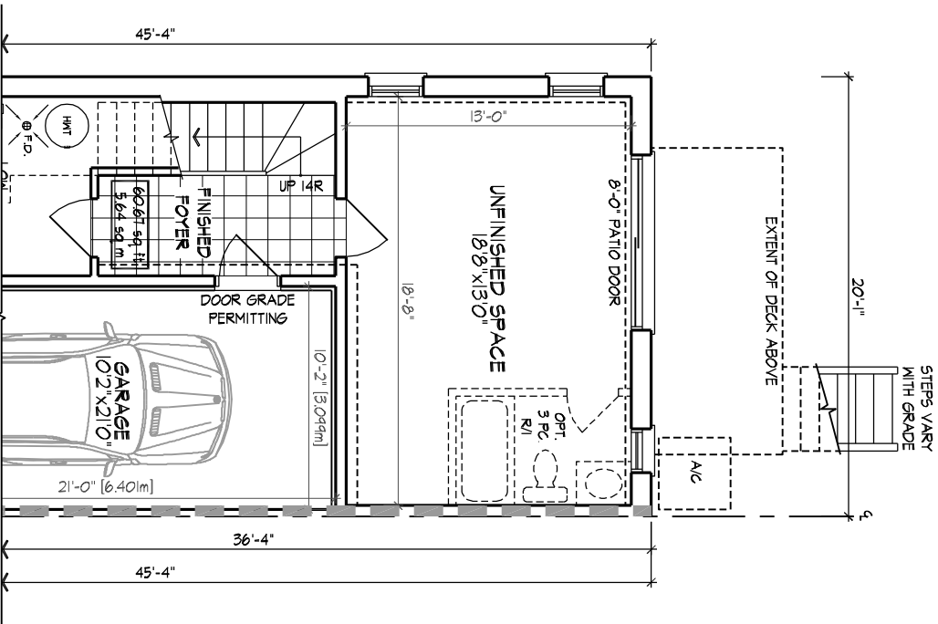
LOOKOUT CONDITION PART. GROUND FLOOR PLAN ELEV. 'A'
