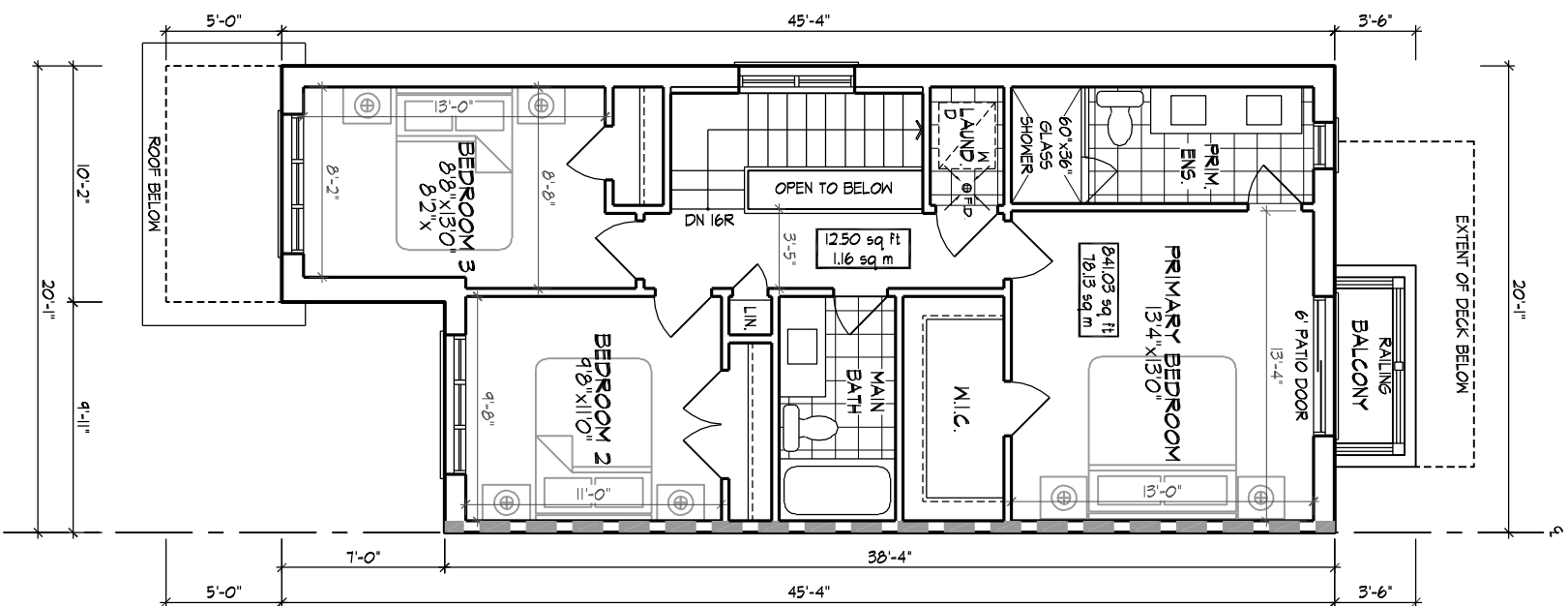
UPPER FLOOR PLAN ELEV. 'A'
