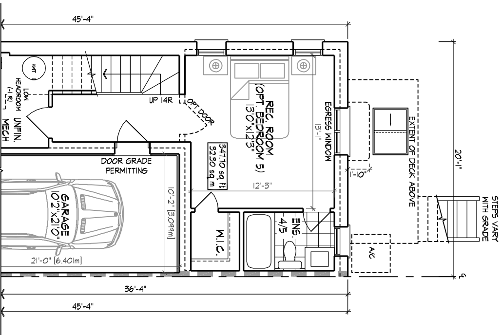
LOOKOUT CONDITION PART. OPT. FINISHED GROUND FLOOR PLAN W/ REC. ROOM/ BEDROOM 4
