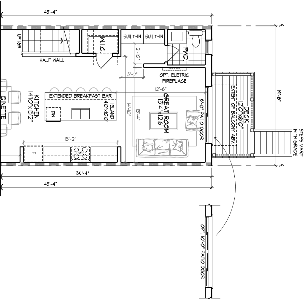
LOOKOUT CONDITION PART. MAIN FLOOR PLAN ELEV. 'A'
