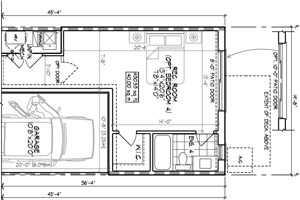
PART. OPT. FINISHED GROUND FLOOR PLAN W/ REC. ROOM/ BEDROOM 4 451 sq ft
