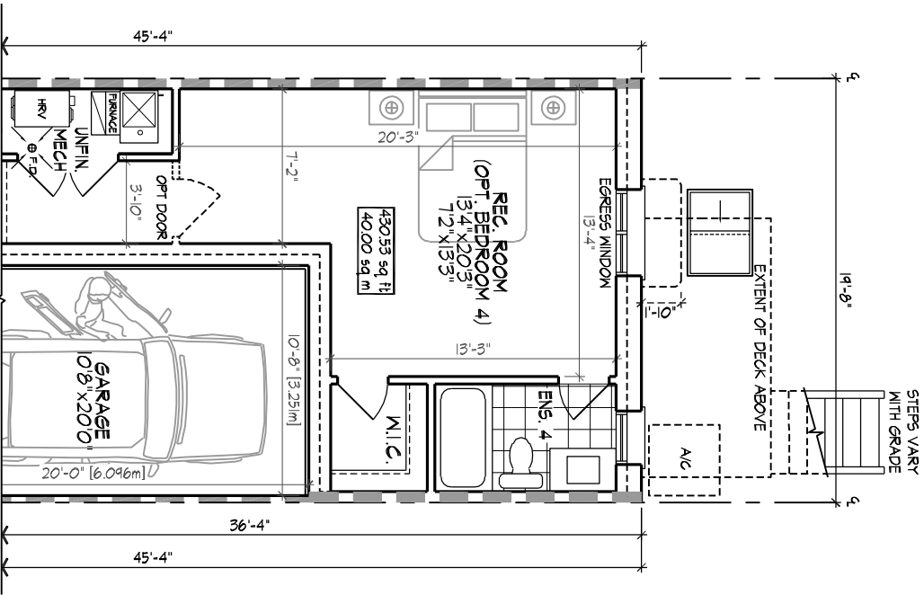
LOOKOUT CONDITION PART. OPT. FINISHED GROUND FLOOR PLAN W/ REC. ROOM/ BEDROOM 4
