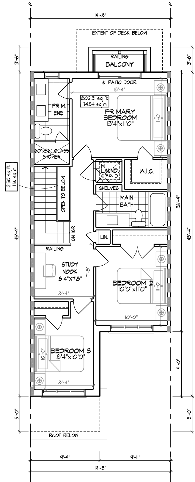
UPPER FLOOR PLAN ELEV. 'A' 790 sq ft GROSS FLOOR AREA 802 sq ft DEDUCT OPEN AREAS 13 sq ft NET AREA 790 sq ft
