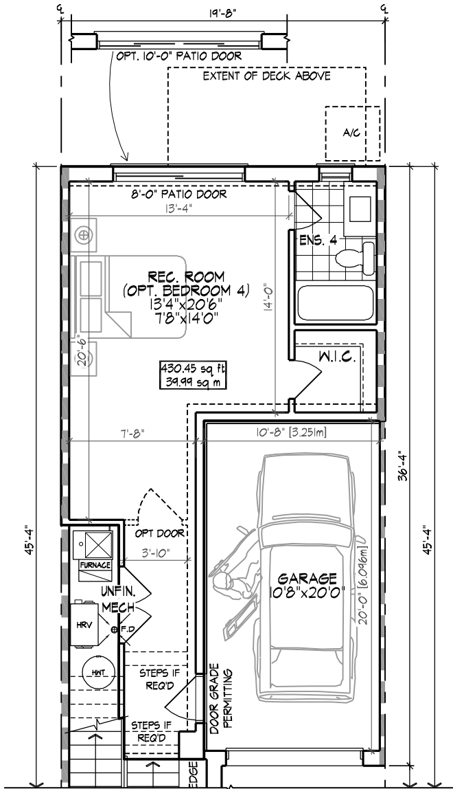
PART. OPT. FINISHED GROUND FLOOR PLAN W/ REC. ROOM/ BEDROOM 4 430 sq ft
