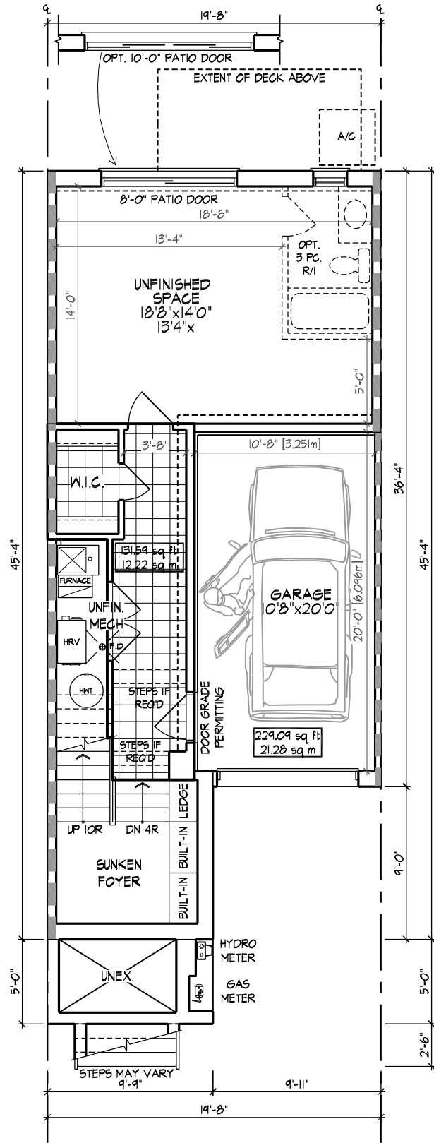
GROUND FLOOR PLAN ELEV. 'A' 132 sq ft COVERAGE W/O PORCH 802 sq ft COVERAGE W/ PORCH 851 sq ft
