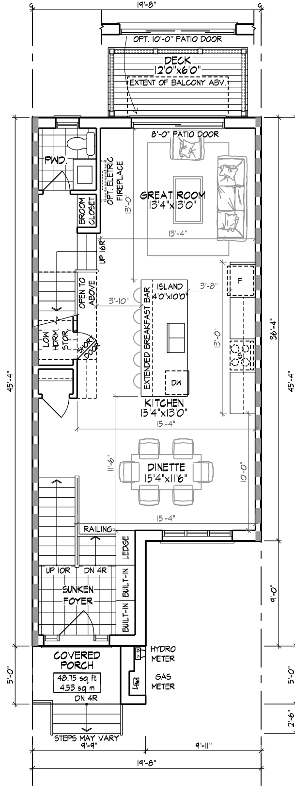
MAIN FLOOR PLAN ELEV. 'A' 802 sq ft GROSS FLOOR AREA 802 sq ft DEDUCT OPEN AREAS 0 sq ft NET AREA 802 sq ft
